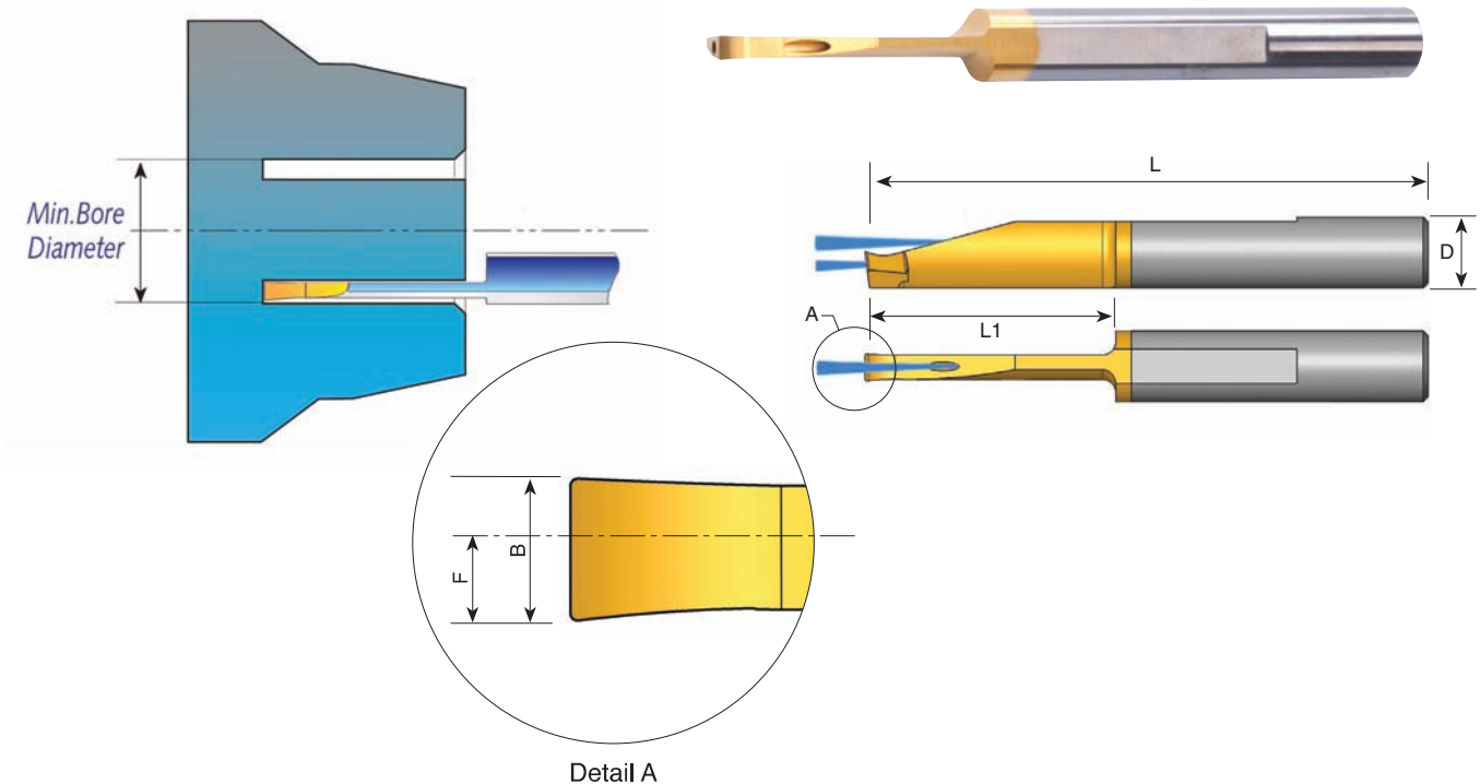
Detail A
